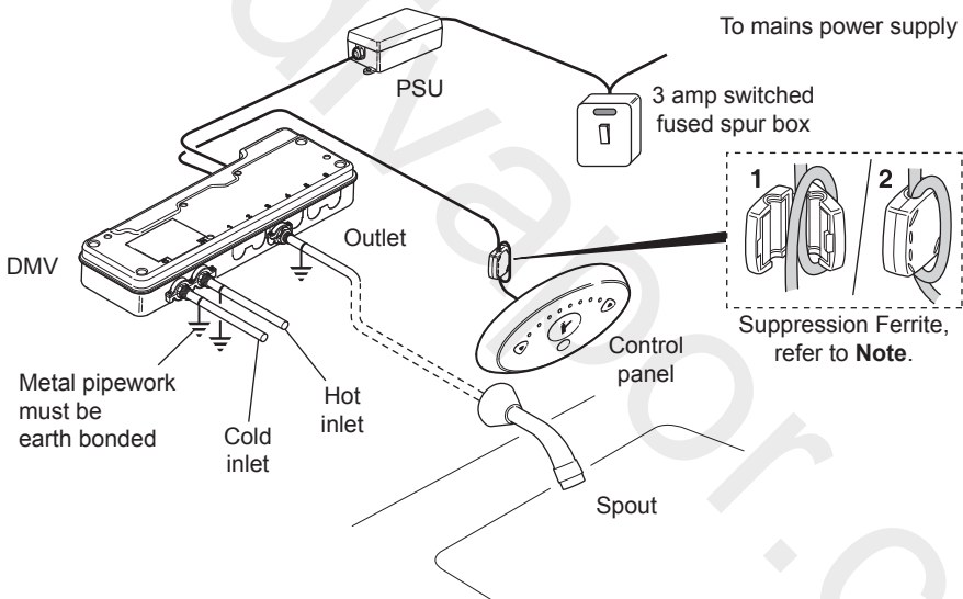
Installation Schematic
