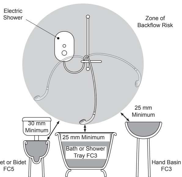
Hose retaining ring fitted and shower fittings fixed at a suitable height preventing dirty water backflow
