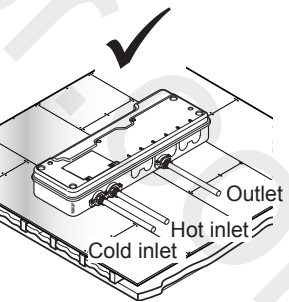
Mounting on a Horizontal Surface
