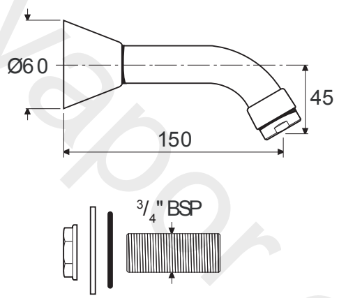
SP T150, Part No. 1503.734
