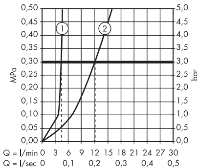
AXOR Uno 2 38020000/38022000/38027000
