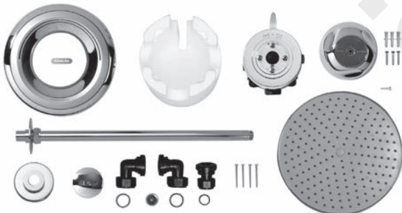
Concealed shower valve with fixed 220mm head
