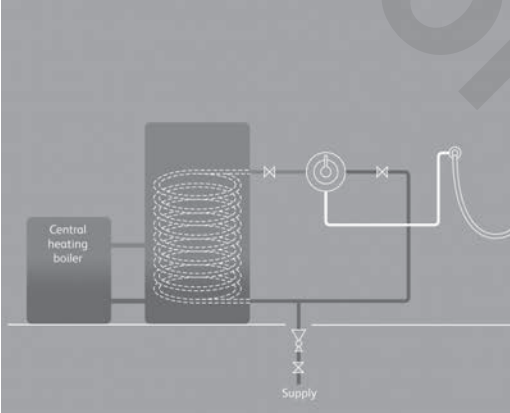
Typical thermal storage unit system installation
