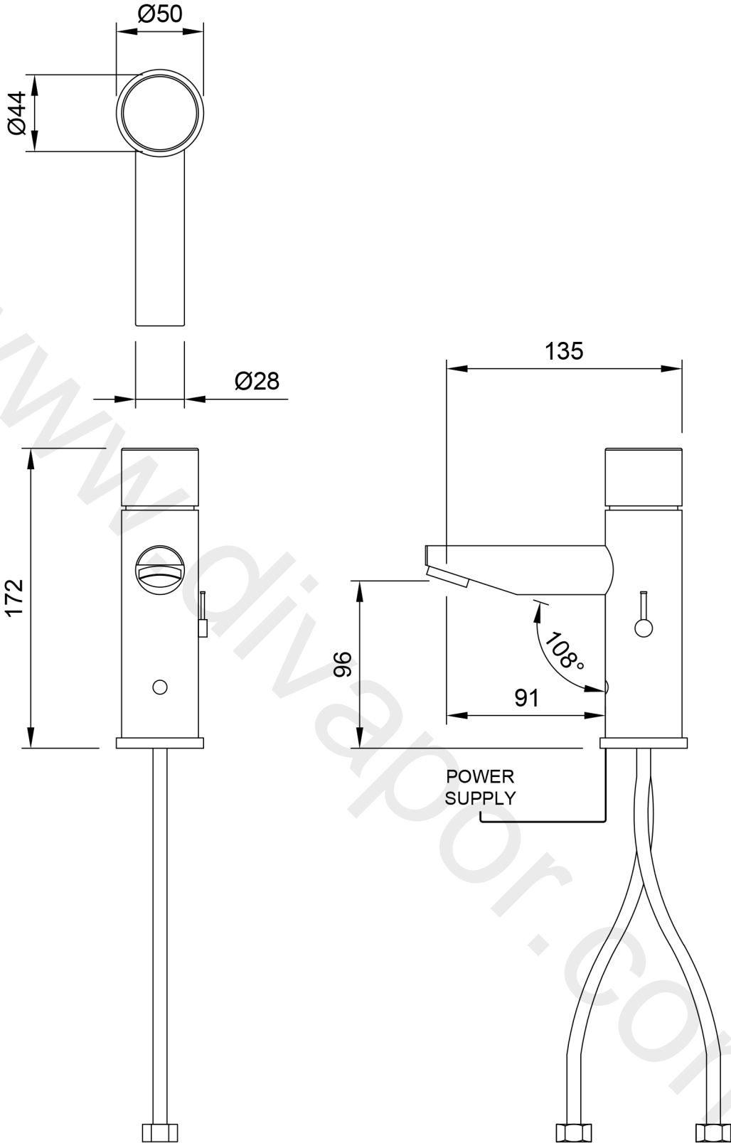
DOLPHIN SOLUTIONS LIMITED DOLPHIN BLUE ELECTRONIC INFRARED TAP WITH TEMPERATURE ADJUSTMENT LEVER DB150/DB175
