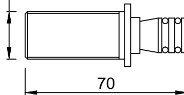
SPOUT NIPPLE
