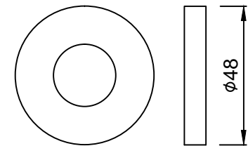
SPOUT SPACER
