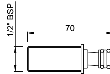
SPOUT NIPPLE
