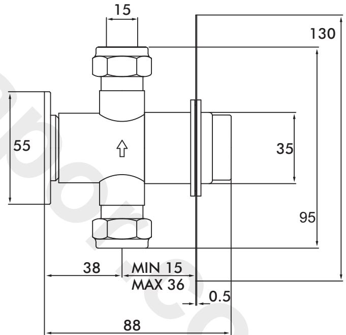
Time Flow Shower Concealed TF997CP
