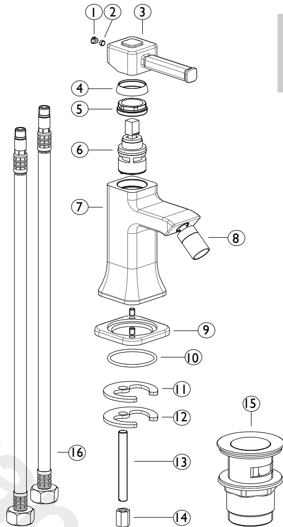
Illustration of bidet mixer only
